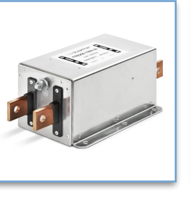
DC Filters
