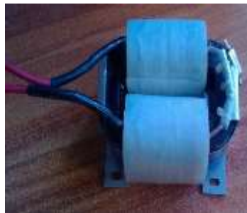
PFC电感 CD16*32*60 115mm*90mm*55mm 6000W 25A 220V
