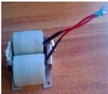
PFC电感 CD12.5*25*60 107mm*72mm*50mm 3000W 15A 220V
